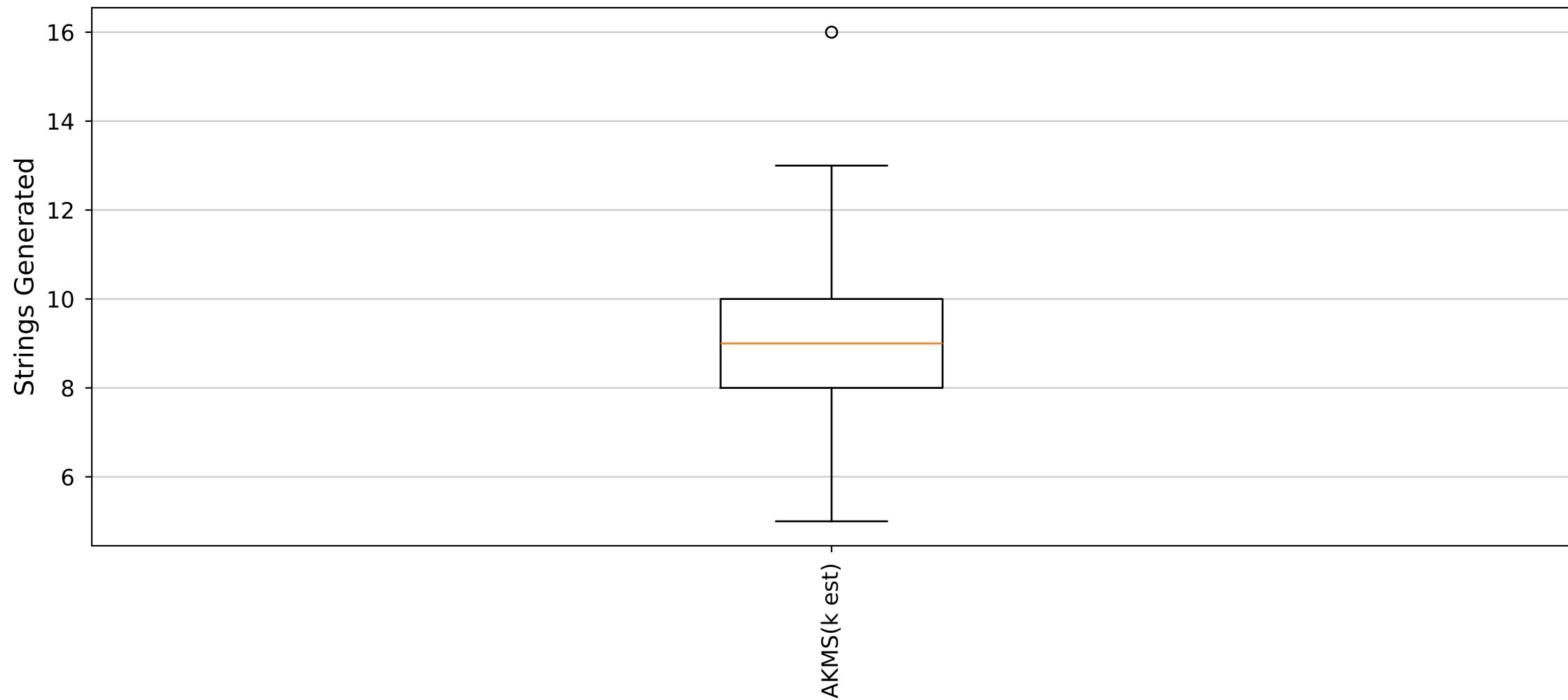
YARA Rules Strings Generated Distribution (Cluster2_Size100 dataset)
